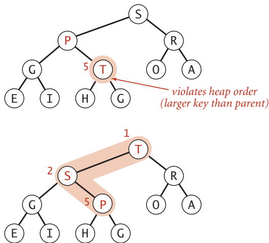
Bottom-up reheapify (swim)
