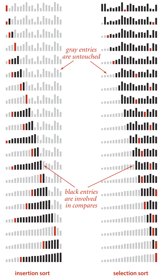
Visual traces of elementary sorting algorithms
