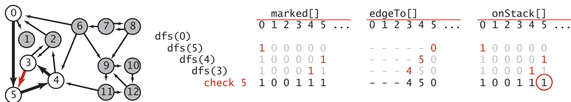
Finding a directed cycle in a digraph
