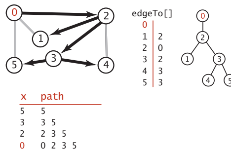
Trace of pathTo(5) computation
