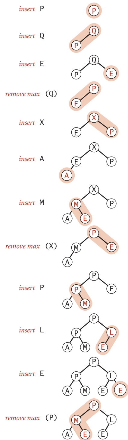
Priority queue operations in a heap
