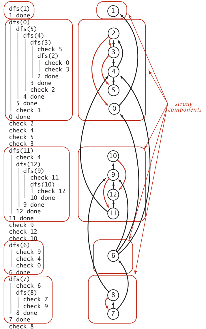
Kosaraju's algorithm for finding strong components in digraphs
