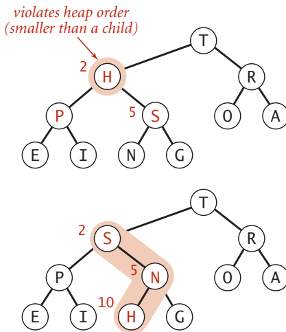
Top-down reheapify (sink)
