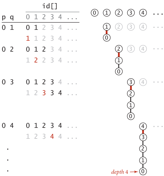
Quick-union worst case
