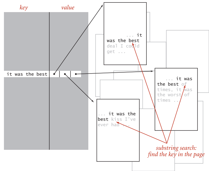
Idealized view of a typical web search
