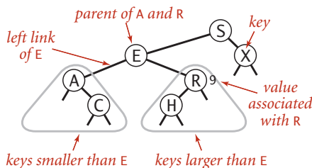
Anatomy of a binary search tree
