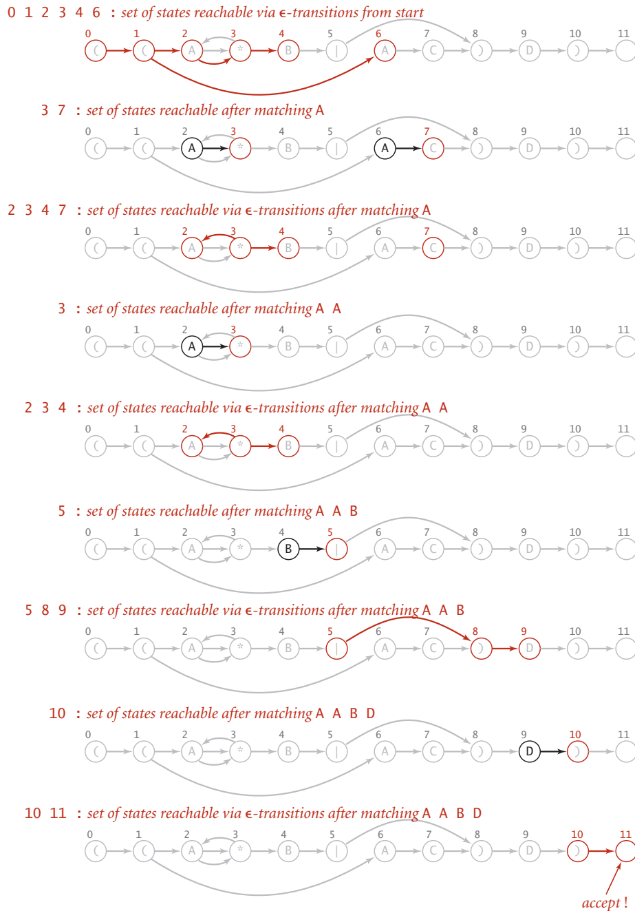
Simulation of C ( A^* B \mid A C ) D NFA for input A A B D
