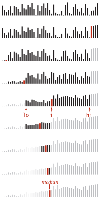
Partitioning to find the median
