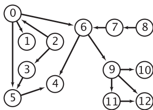
Standard digraph model
