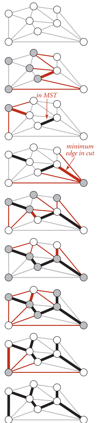
Greedy MST algorithm
