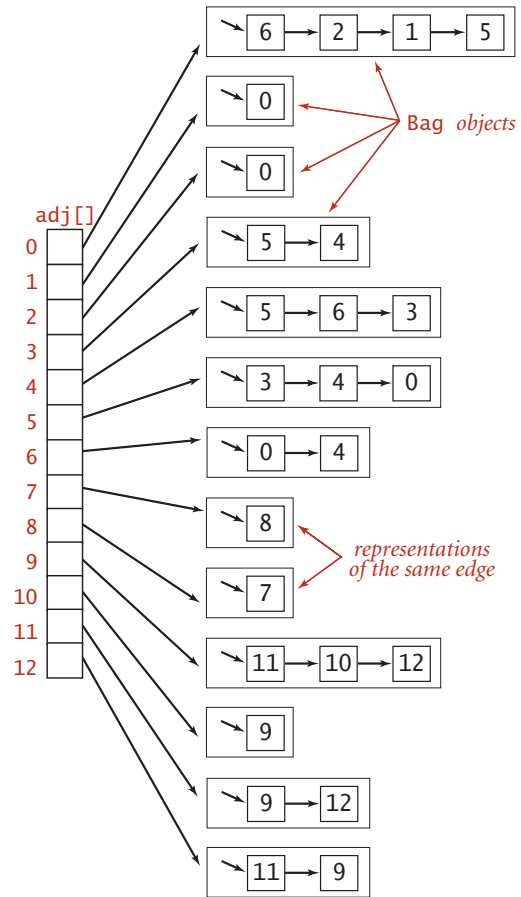
Adjacency-lists representation (undirected graph)
