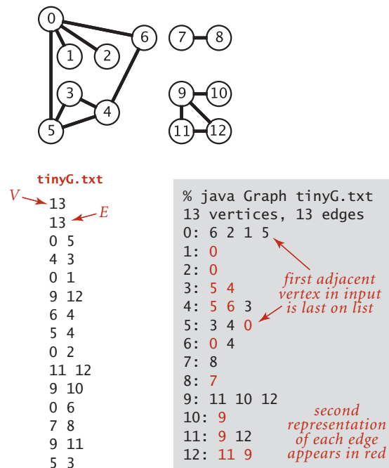
Output for list-of-edges input
