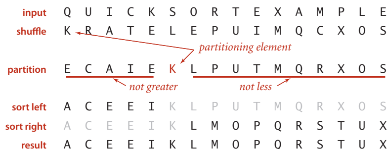
Quicksort overview
