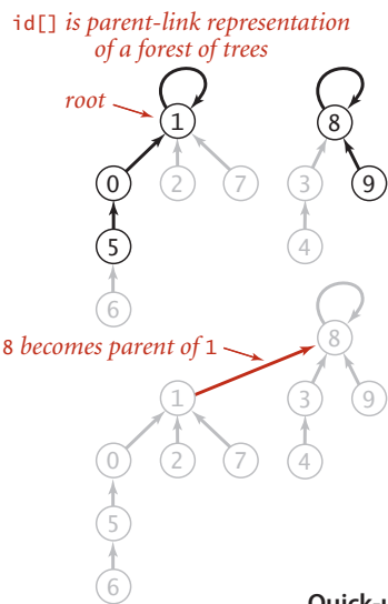
Quick-union overview
