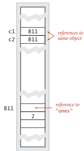
Aliasing
