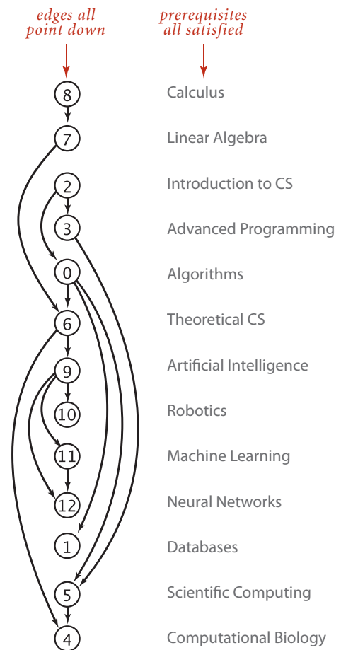
Topological sort
