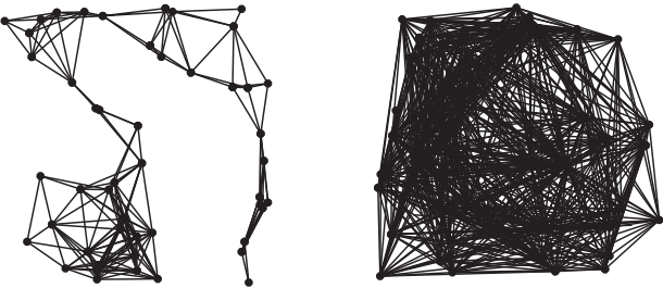
Two graphs ( V = 50 )
