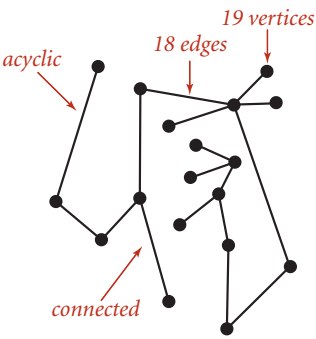
A tree
