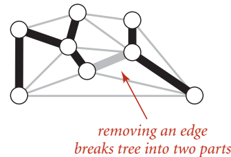
Basic properties of a tree
