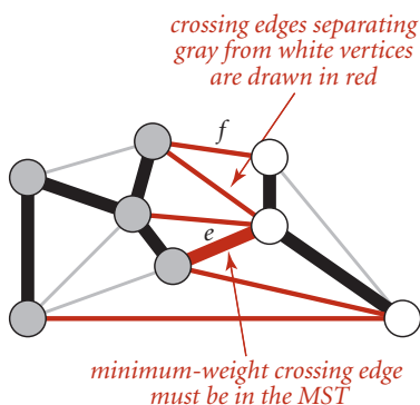
Cut property
