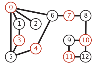
A bipartite graph
