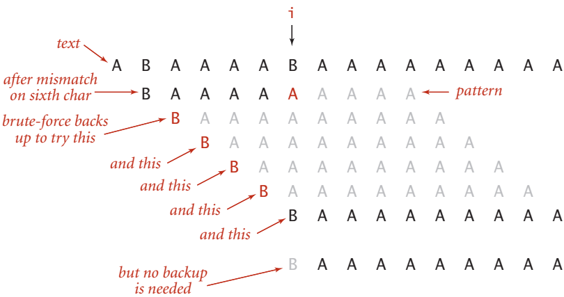
Text pointer backup in substring searching
