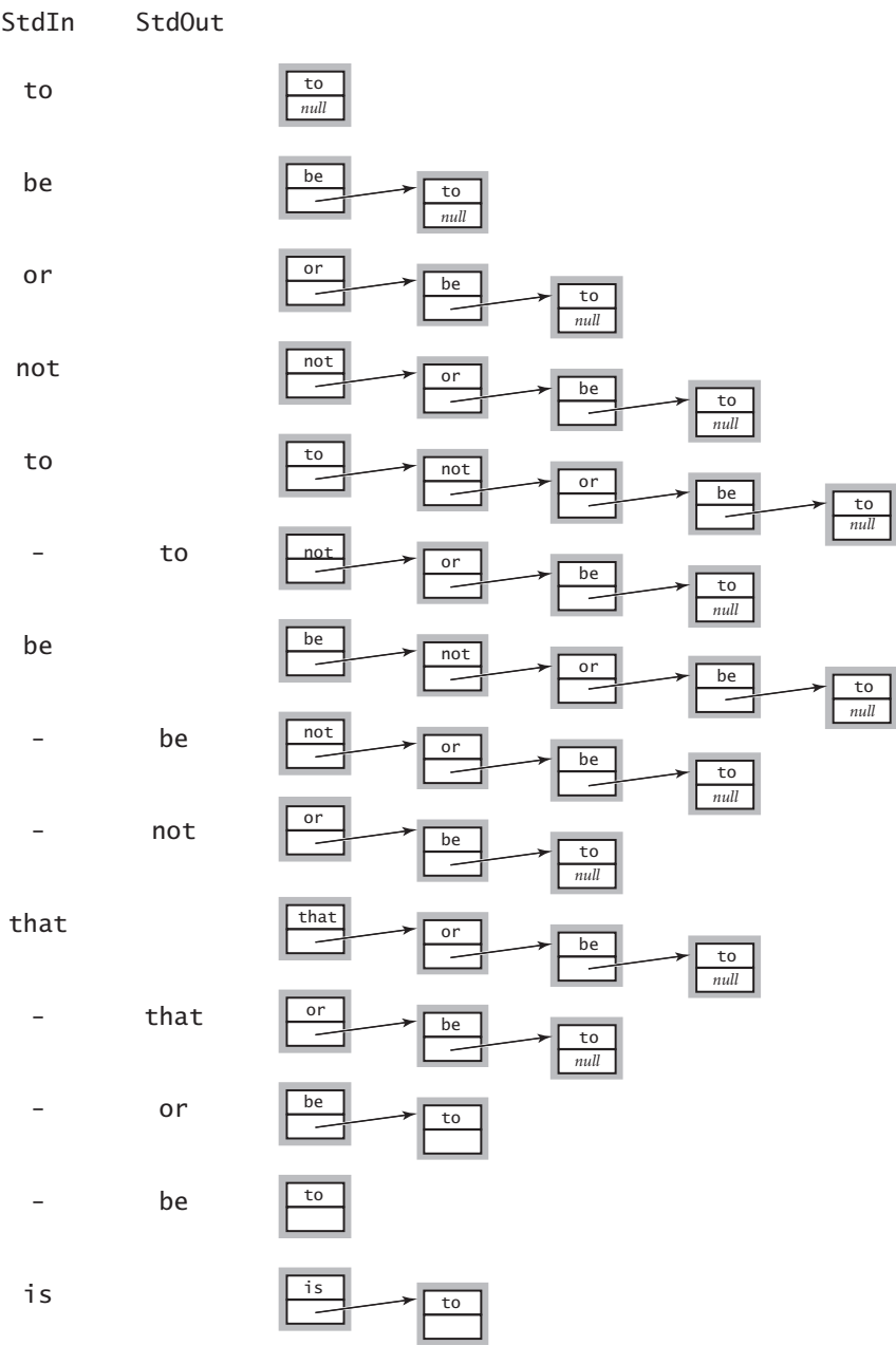
Trace of Stack development client
