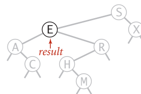
Computing the floor function
