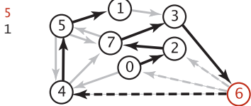
Trace of the Bellman-Ford algorithm (negative weights)
