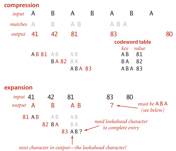
LZW expansion: tricky situation
