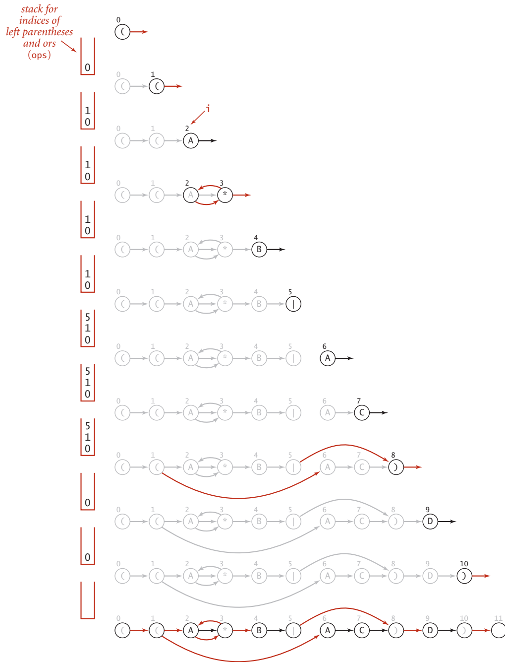
Building the NFA corresponding to ((A * B | A C) D)
