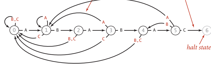
DFA corresponding to the string A B A B A C
