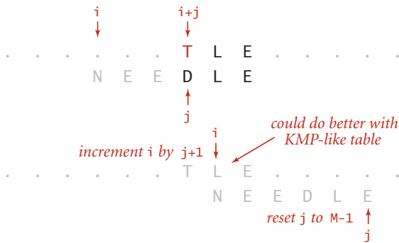
Mismatched character heuristic (mismatch not in pattern)
