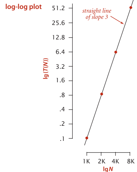
Analysis of experimental data (the running time of ThreeSum.count() )
