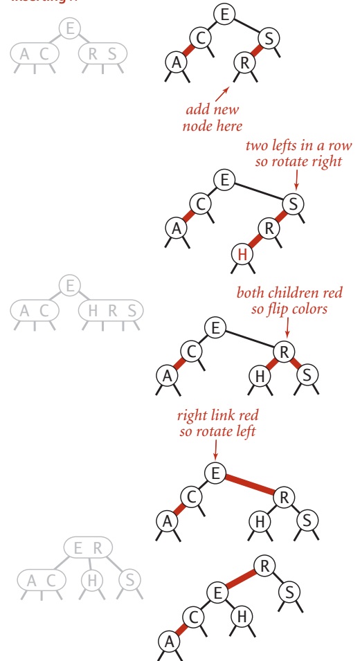
Insert into a 3-node at the bottom
