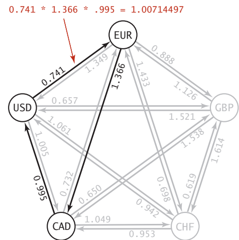
An arbitrage opportunity
