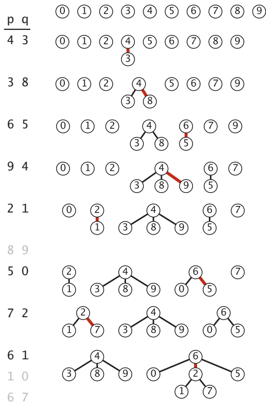
Weighted quick-union traces (forests of trees)
