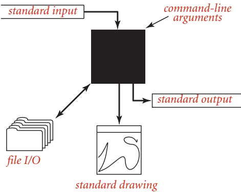
A bird's-eye view of a Java program
