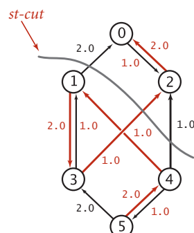
Trace of augmenting-path Ford-Fulkerson algorithm
