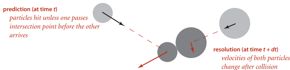
Predicting and resolving a particle-particle collision
