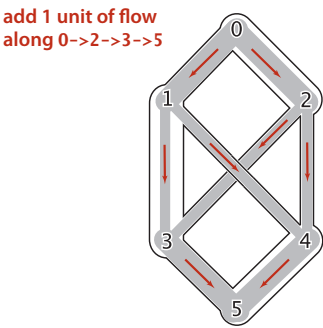
Adding flow to a network
