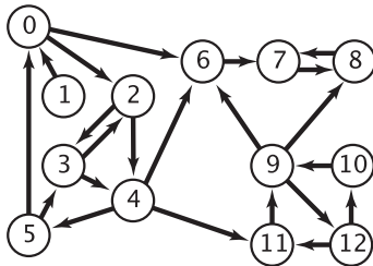
DFS in reverse digraph (ReversePost)
