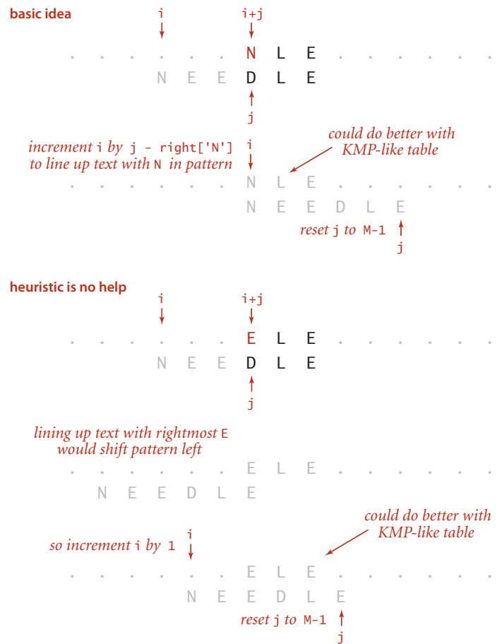
Mismatched character heuristic (mismatch in pattern)
