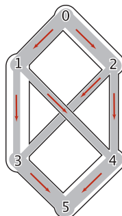
Trace of augmenting-path Ford-Fulkerson algorithm
