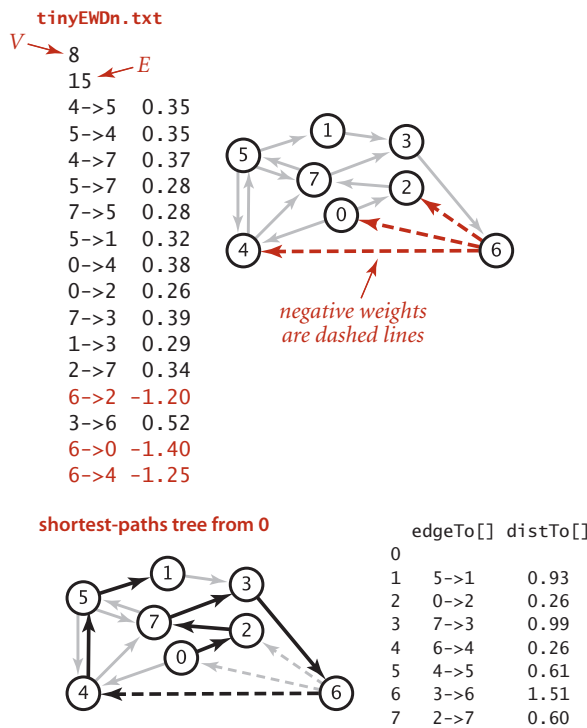
An edge-weighted digraph with negative weights
