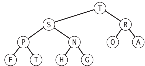
A heap-ordered complete binary tree
