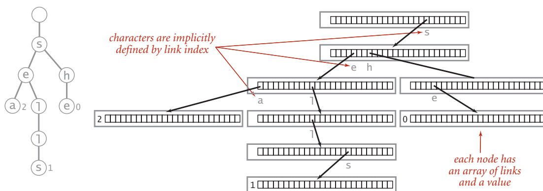
Trie representation ( R = 26 )
