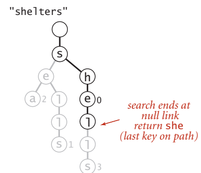
Possibilities for longestPrefixOf()
