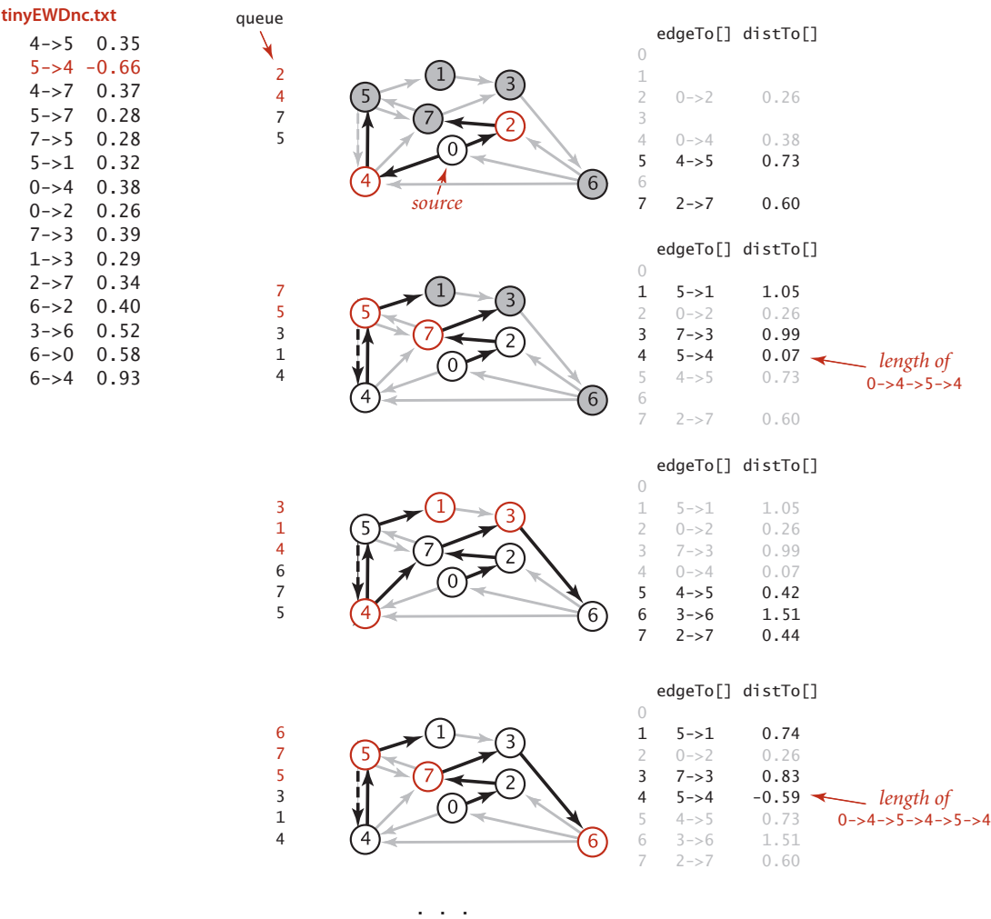
Trace of the Bellman-Ford algorithm (negative cycle)
