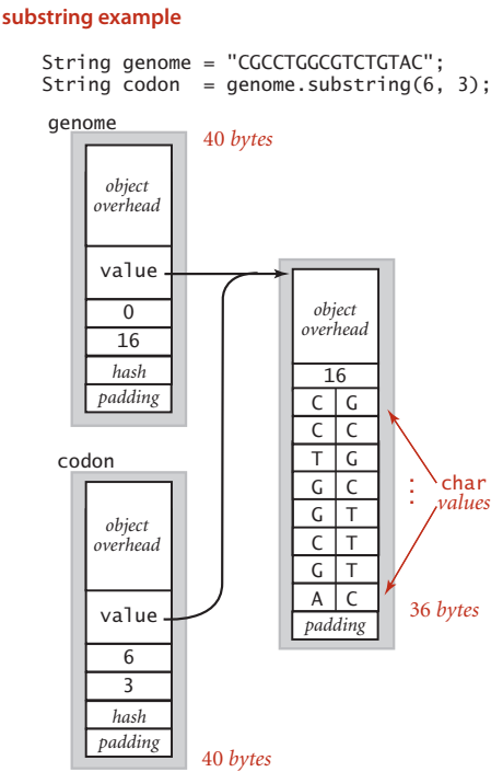
A String and a substring
