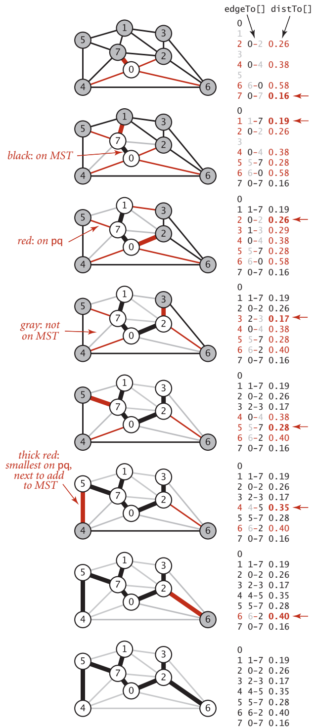
Trace of Prim's algorithm (eager version)
