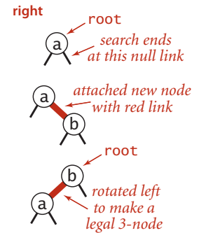
Insert into a single 2-node (two cases)
