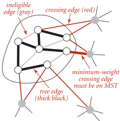
Prim's MST algorithm
