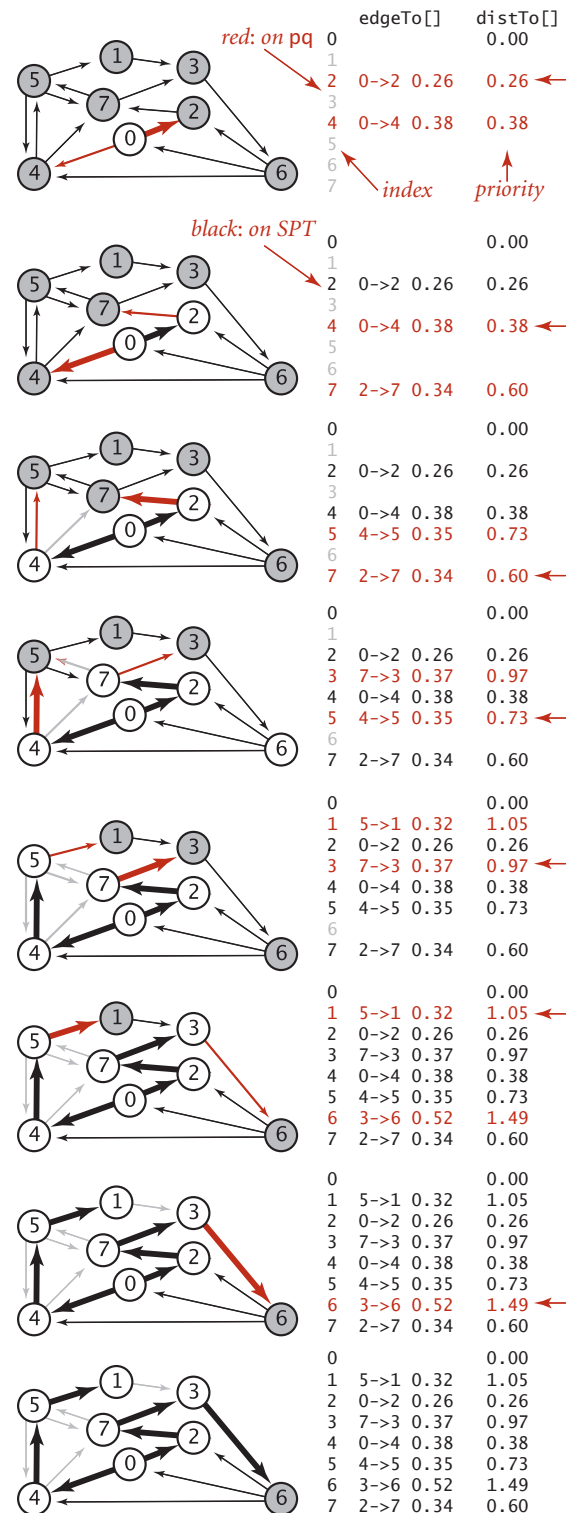
Trace of Dijkstra's algorithm
