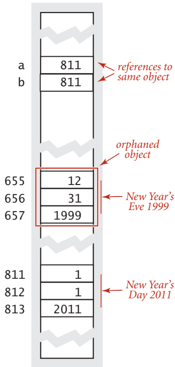
An orphaned object
