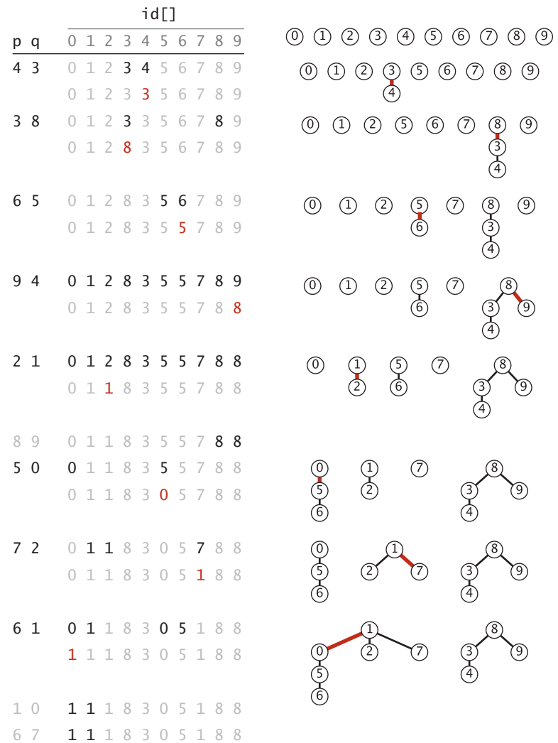
Quick-union trace (with corresponding forests of trees)
