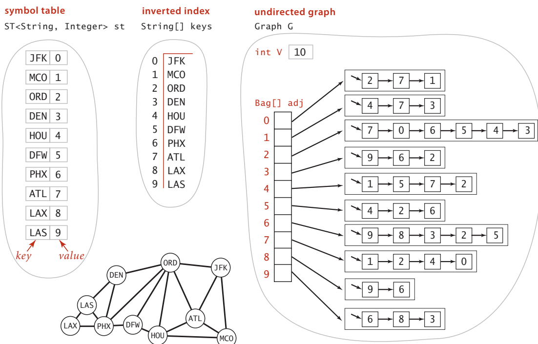
Symbol graph data structures
