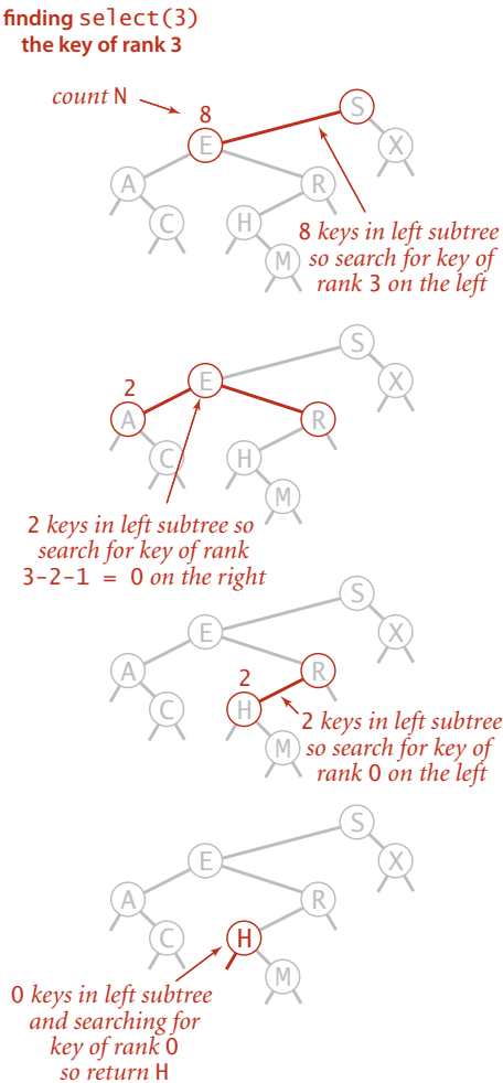
Selection in a BST
