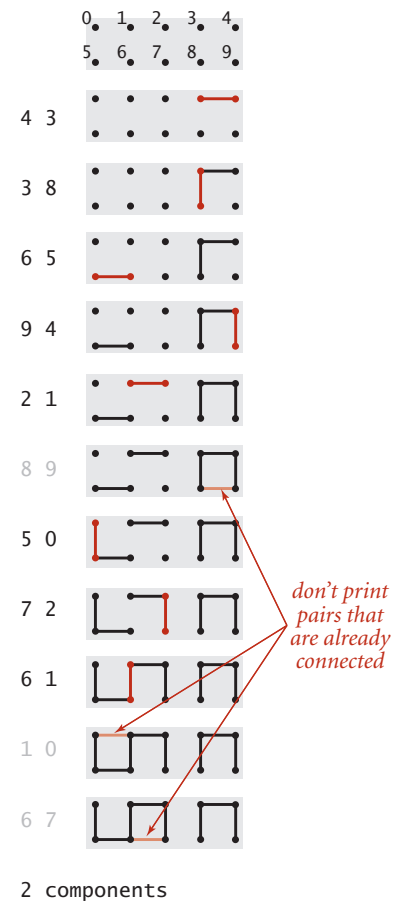
Dynamic connectivity example
