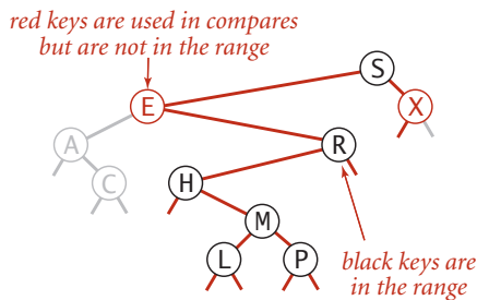
Range search in a BST
