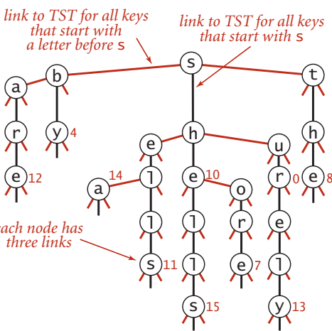
TST representation of a trie
