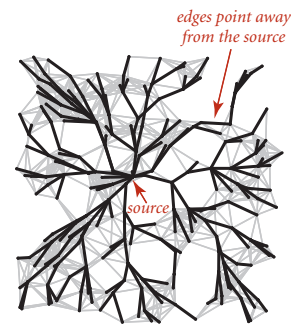
An SPT with 250 vertices
