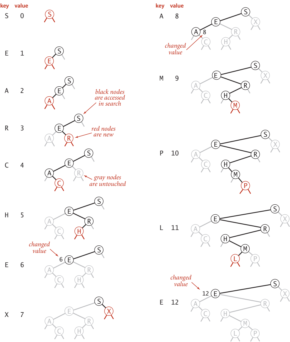
BST trace for standard indexing client
