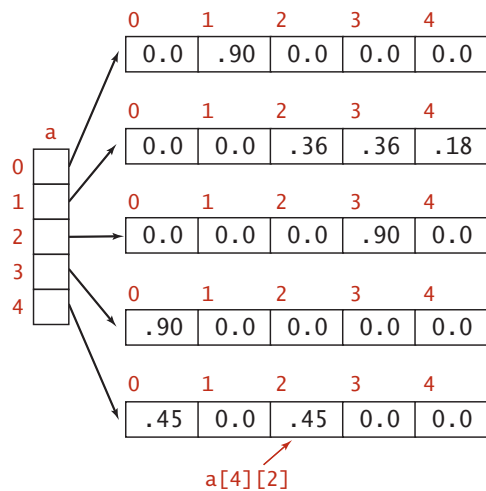
array of double[] objects
