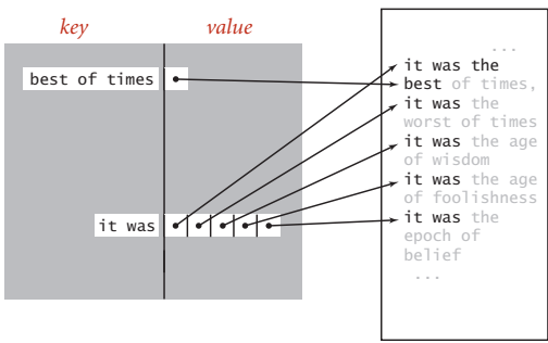
Idealized view of a text-string index
