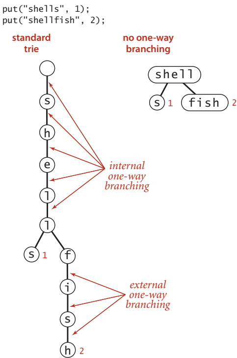
Removing one-way branching in a trie
