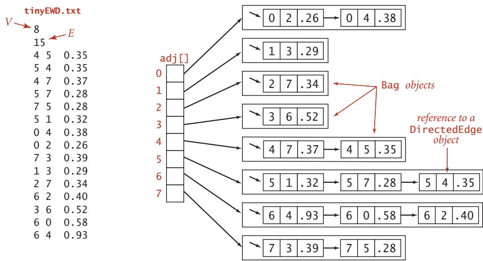
Edge-weighted digraph representation
