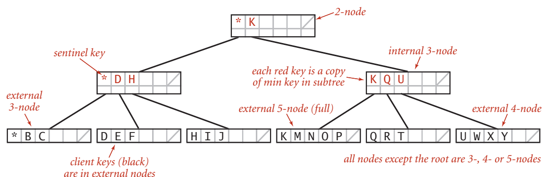
Anatomy of a B-tree set ( M = 6 )
