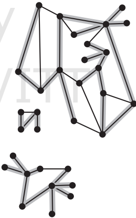
A spanning forest
