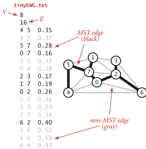
An edge-weighted graph and its MST
