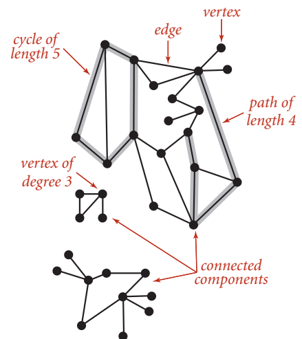
Anatomy of a graph
