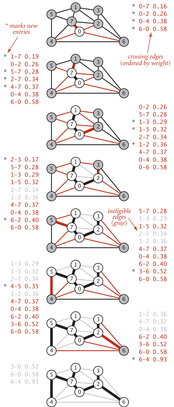
Trace of Prim's algorithm (lazy version)
