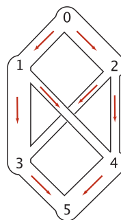
Anatomy of a network-flow problem
