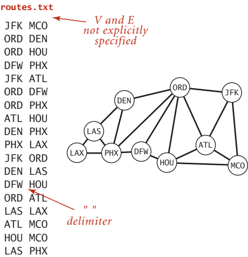
Symbol graph example (list of edges)
