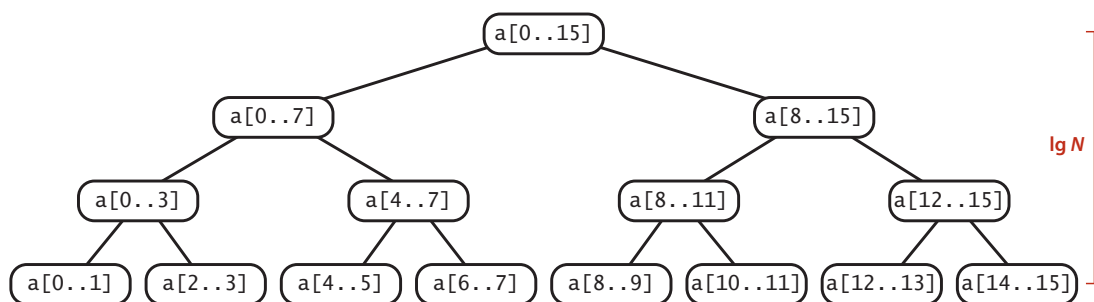
Mergesort subarray dependence tree for N = 16
