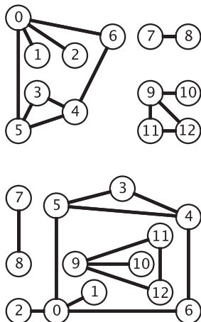
Two drawings of the same graph
