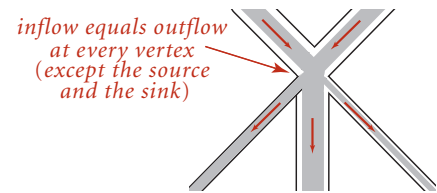
Local equilibrium in a flow network
