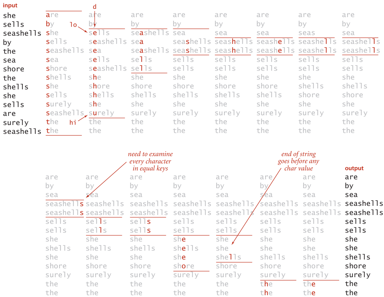
Trace of recursive calls for MSD string sort (no cutoff for small subarrays, subarrays of size 0 and 1 omitted)
