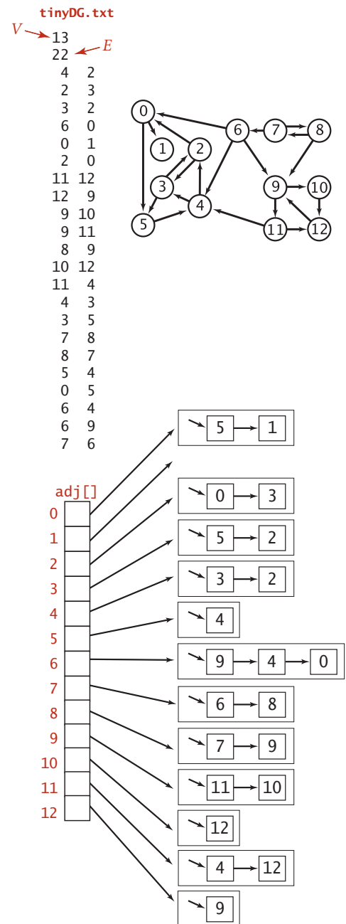
Digraph input format and adjacency-lists representation
