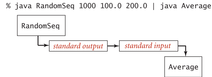
Redirection and piping from the command line
