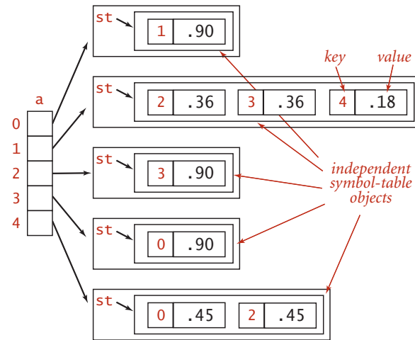
Sparse matrix representations
