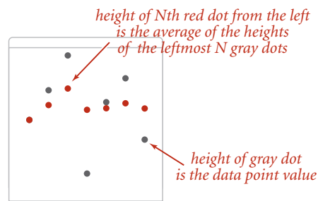
Visual accumulator plot
