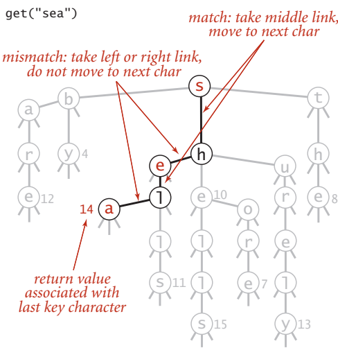
TST search example
