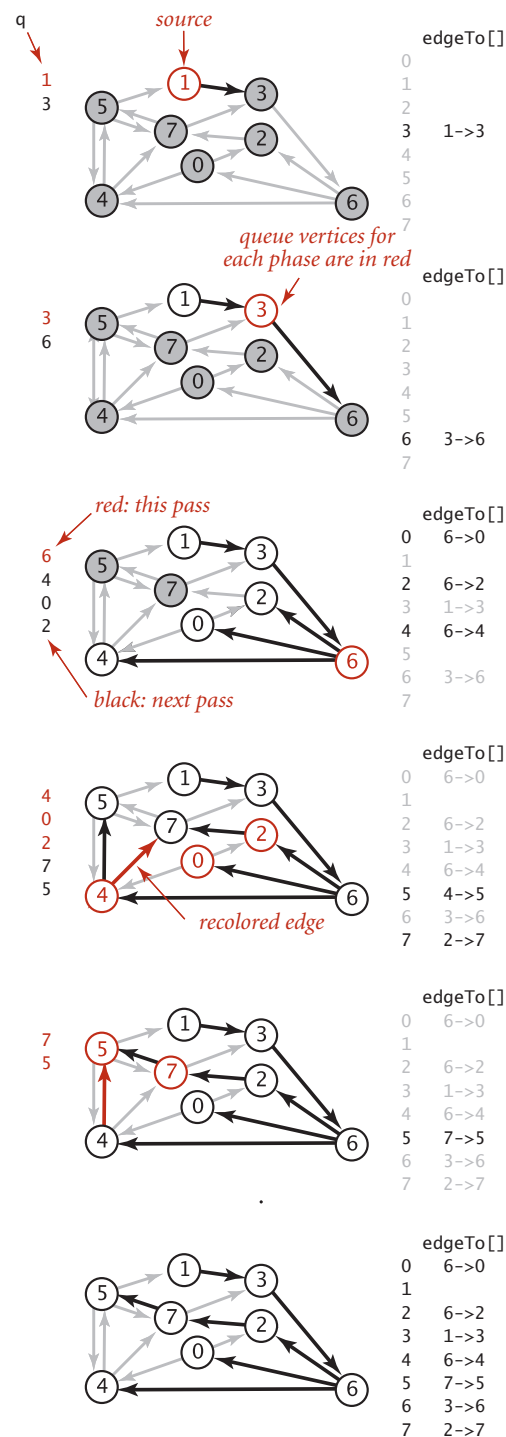
Trace of the Bellman-Ford algorithm
