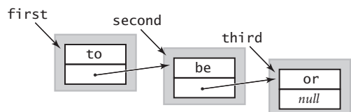
Linking together a list
