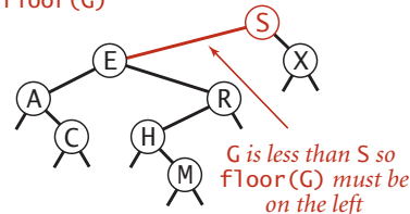
finding floor(G)
