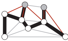
A cut with two MST edges
