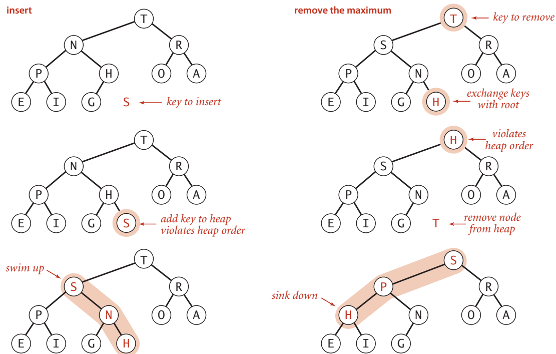
Heap operations
