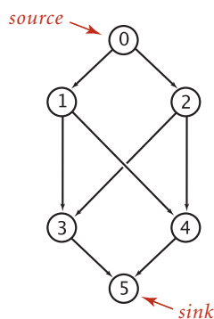
standard drawing
