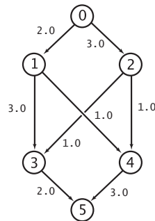
residual network
