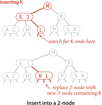
inserting K
