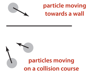
Predictable events
