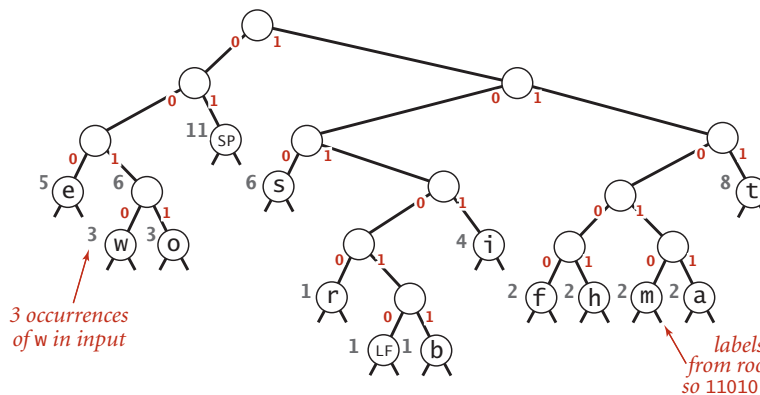
trie representation
