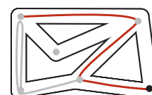
Tremaux exploration
