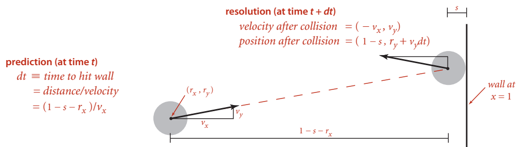
Predicting and resolving a particle-wall collision
