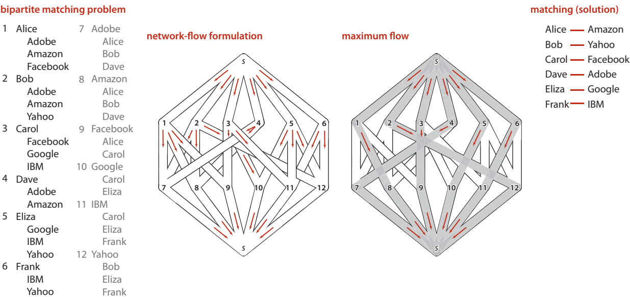
Example of reducing maximum bipartite matching to network flow
