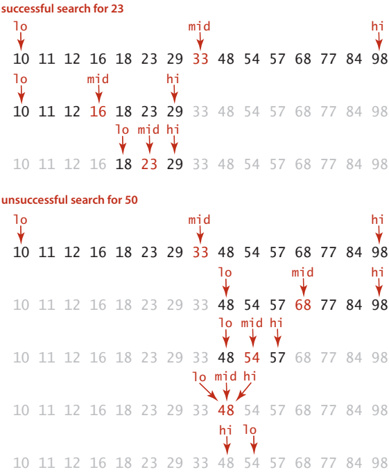
Binary search in an ordered array
