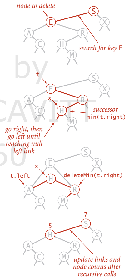
Deletion in a BST
