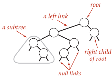
Anatomy of a binary tree
