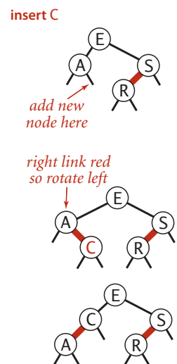
Insert into a 2-node at the bottom
