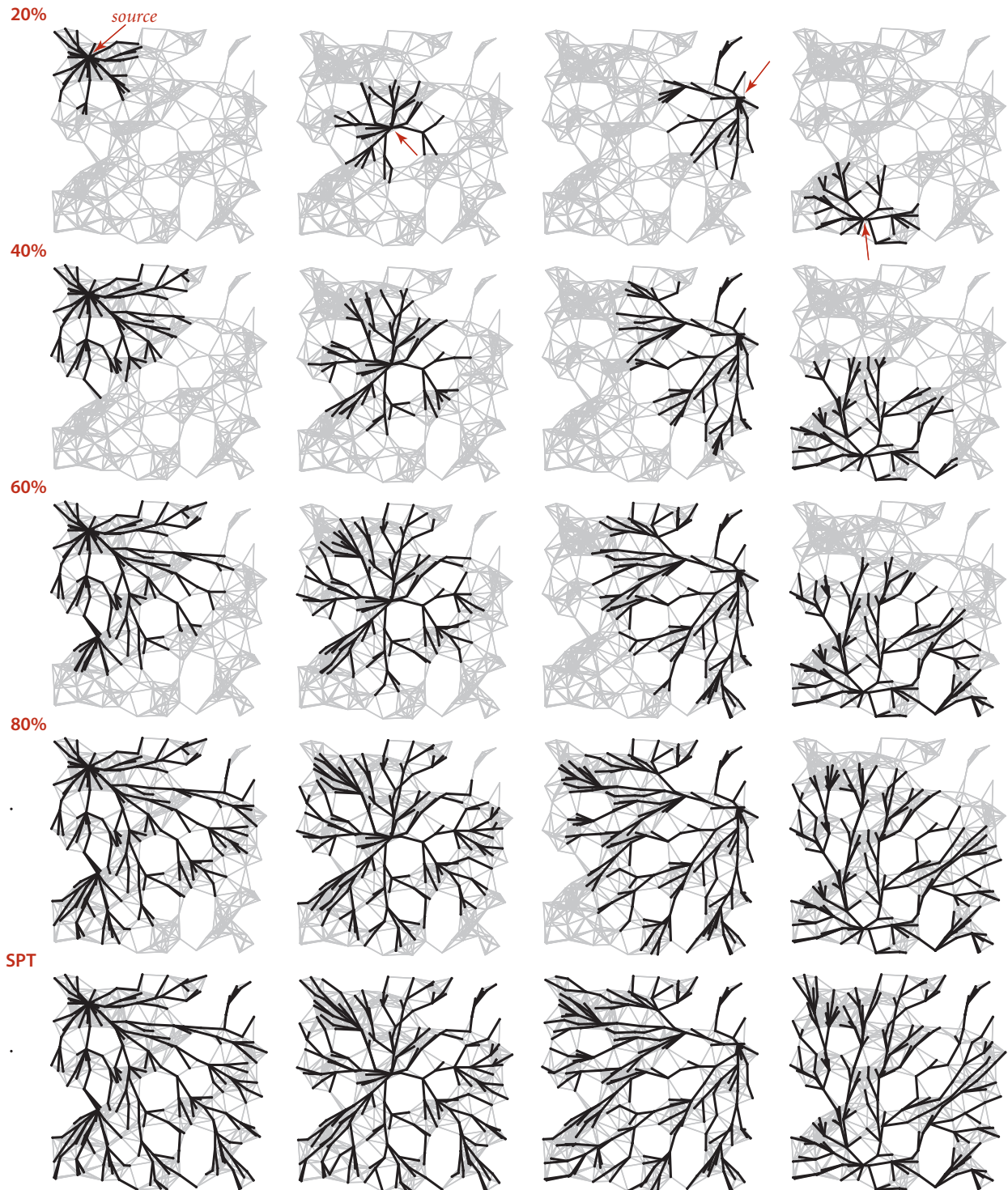
Dijkstra's algorithm (250 vertices, various sources)
