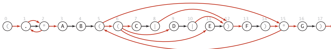
NFA corresponding to the pattern (.*AB((C|D|E)F)^*G)
