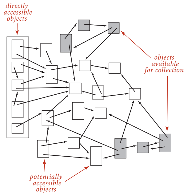
Garbage collection scenario
