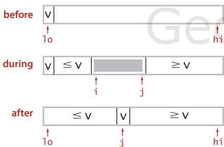
QuickSort partitioning overview
