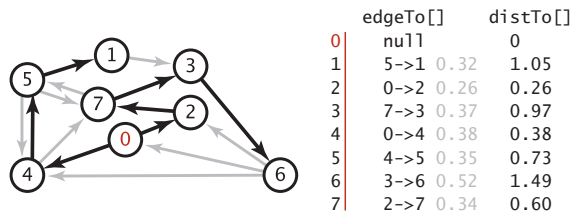
Shortest-paths data structures
