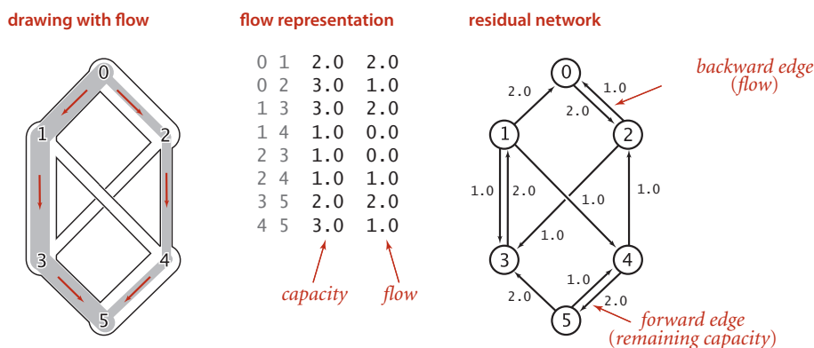
Anatomy of a network-flow problem (revisited)
