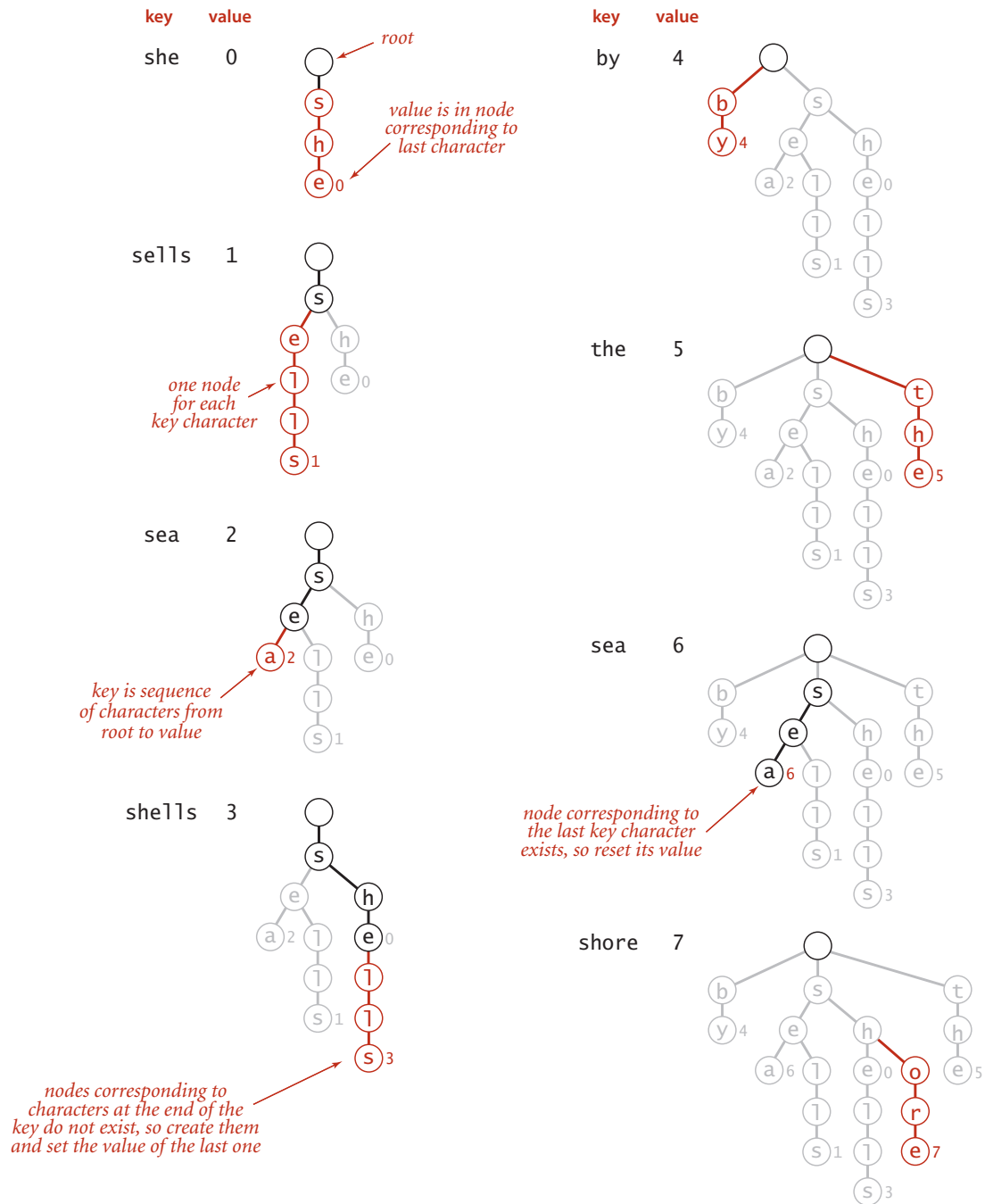
Trie construction trace for standard indexing client
