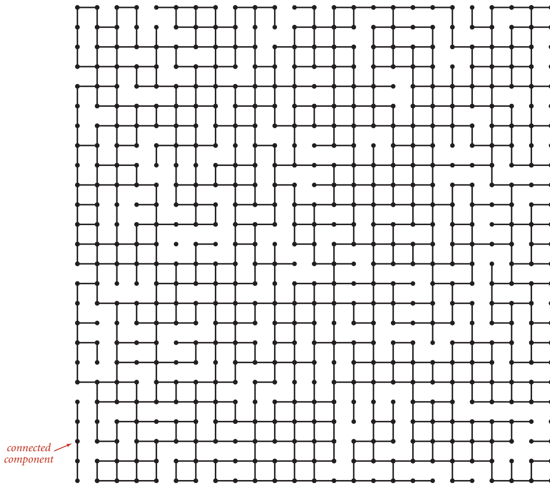
Medium connectivity example (625 sites, 900 edges, 3 connected components)
