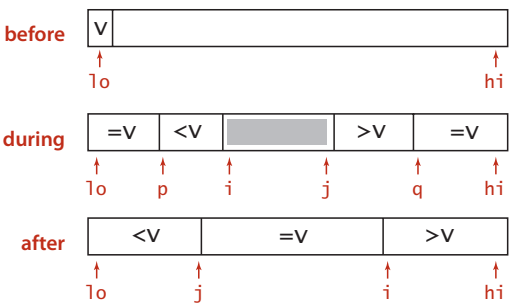
Bentley-McIlroy 3-way partitioning
