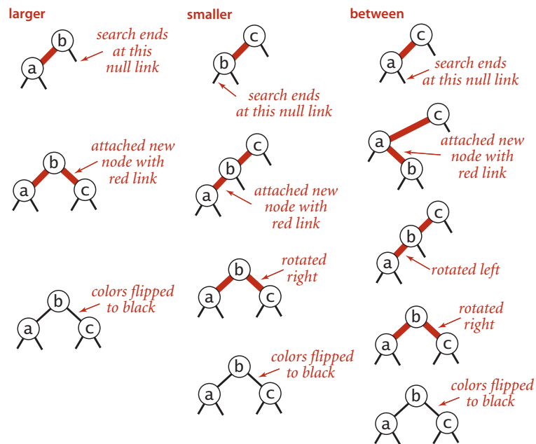
Insert into a single 3-node (three cases)
