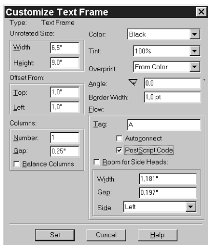
Fig. 6.3. Defining a PostScript frame in FrameMaker
