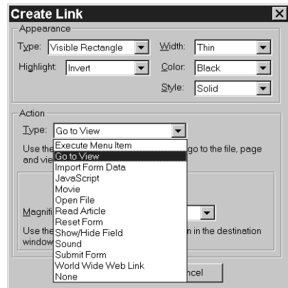
Fig. 6.5. All of the actions which can be defined in Exchange using a link, a bookmark, or a page action can also be defined using pdfmarks.
