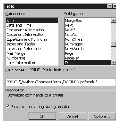
Fig. 6.4. pdfmark code in a Microsoft Word print field
