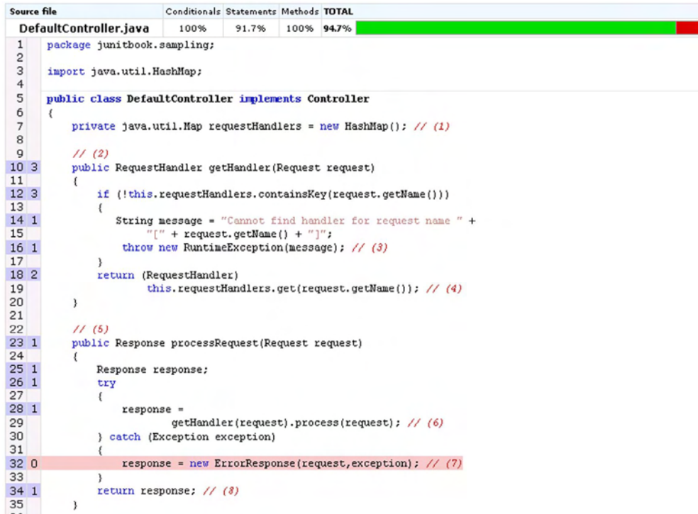
Figure 4.8 A Clover report showing how many times lines of code have been tested and what portion of the code has not been tested (line 32)
