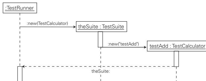
Figure 2.8 JUnit creates an automatic test suite (when the suite method is not defined in the test case).
