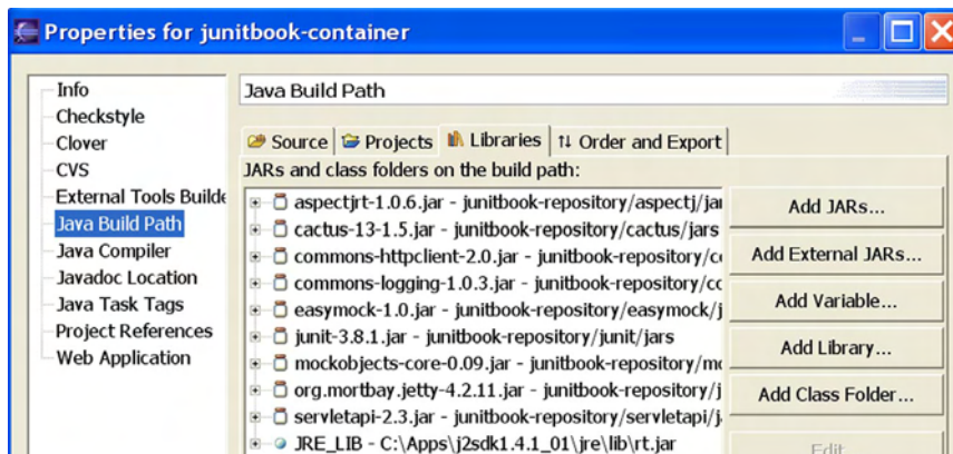
Figure 8.6 Jars required for the junitbook-container project in Eclipse
