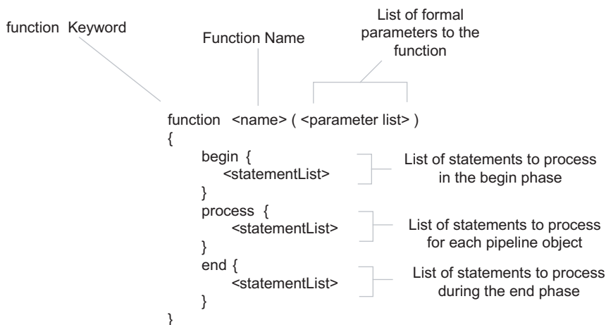
Figure 7.4 This shows the complete function definition syntax for a function in PowerShell that will have cmdlet-like behavior.
