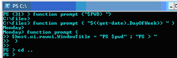
Figure A.1 Setting in the prompt in PowerShell
